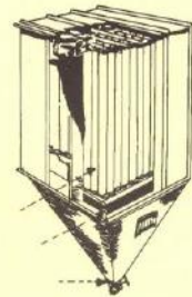
SHAKER CLEANED FILTERS (REVERSE FLOW CLEANED)
